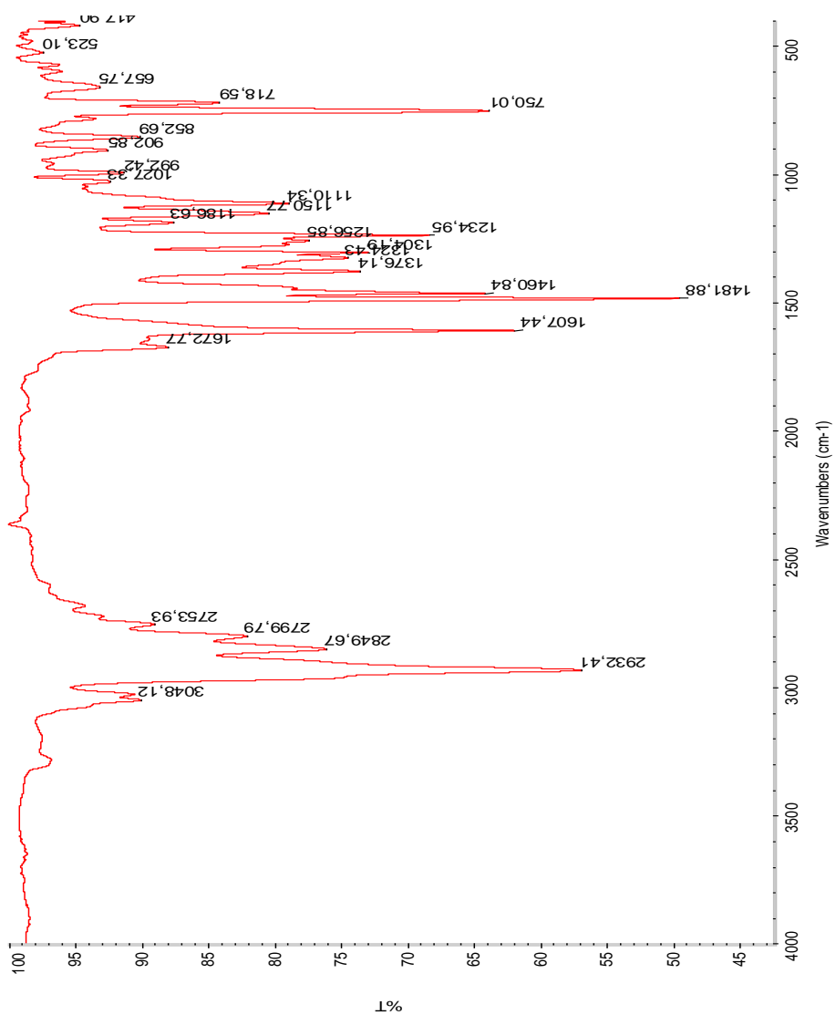
Figure 54: IR spectrum of (AZ-5).
